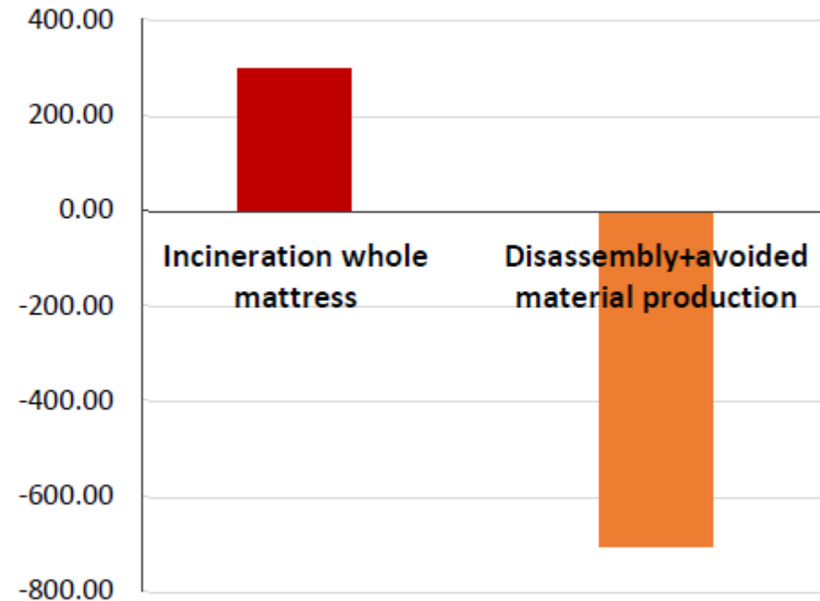
Whole mattress scenarios emissions (kg CO 2 -eq)
